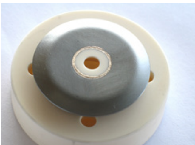
Active-brazed focus electrode made of \text{Al}_2\text{O}_3 ceramic and tantalum (Listemann AG, Eschen/LI)
