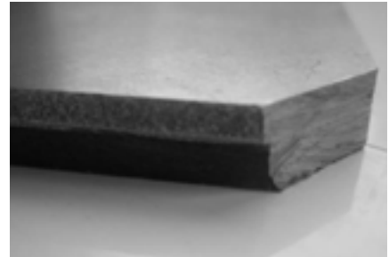
Brazed composite sheet element (Euromat GmbH, Baesweiler)
