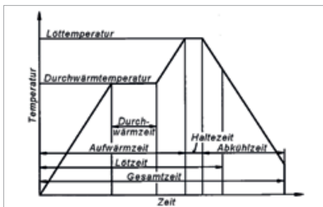
Figure 1: temperature-time diagram
